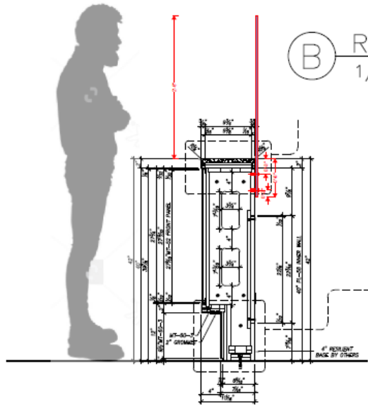
Ⓒ RAC COUNTER — TRANSACTION COUNTER VERTICAL SECTION 3/4" = 1'-0" Arch. Ref. 30 AR 972/ 12
