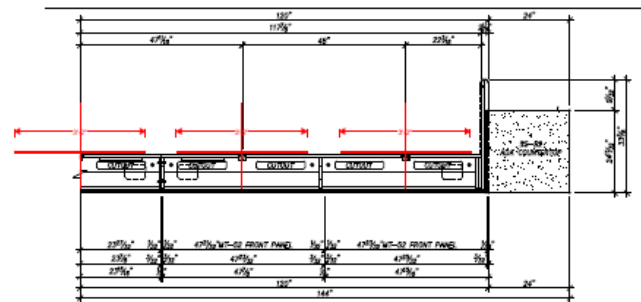
Ⓓ RAC COUNTER — PLAN SECTION 1" = 1'-0" Arch. Ref. N/A
